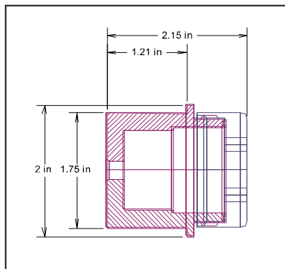
Figure 1. Probe dimensions
