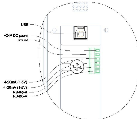
Figure 6 Electrical connections, viewed from the analyzer side
