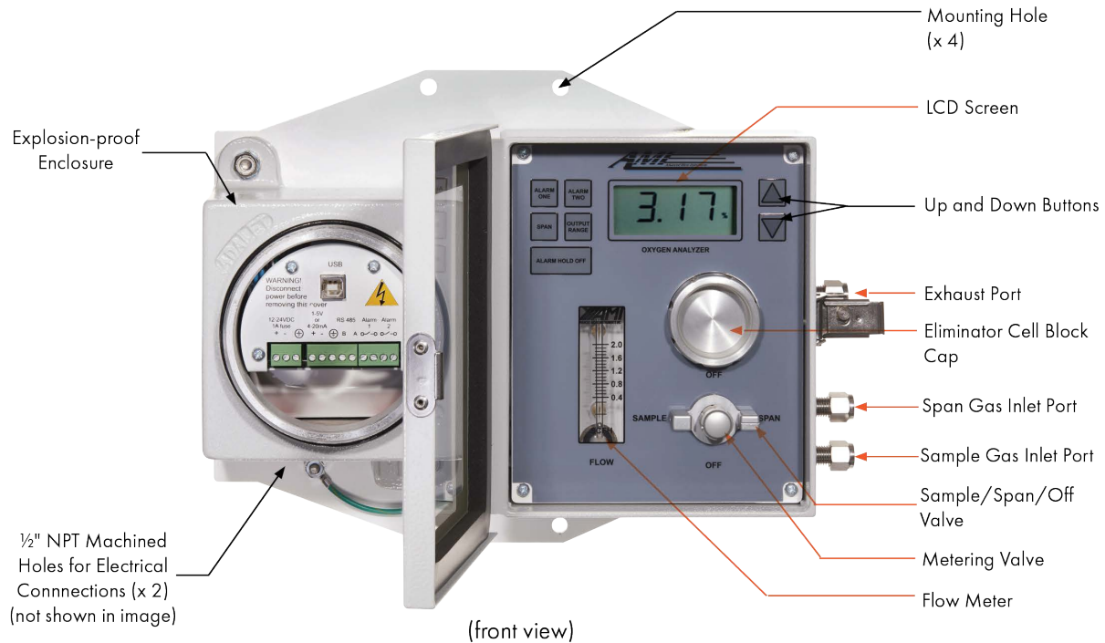
Figure 6. Analyzer without lid
