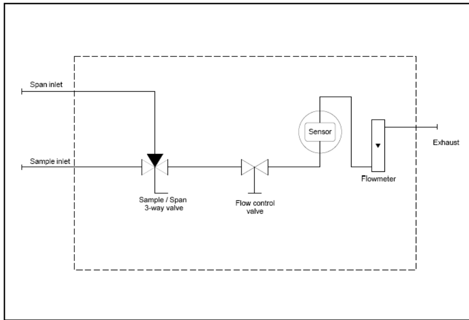
Figure 8. Flow schematic
